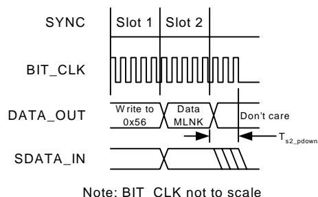
Figure 7. AC-Link Low Power Mode Timing Diagram
