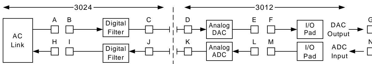
Figure 29. Loopback Points
