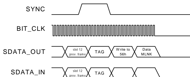
Figure 28. AC-Link Powerdown Timing
