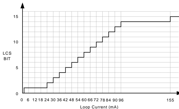
Figure 22. Typical LCS Transfer Function
