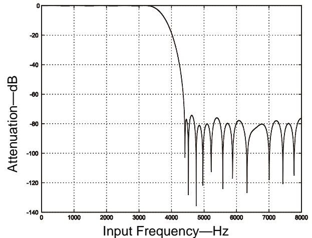
Figure 11. FIR Transmit Filter Response
