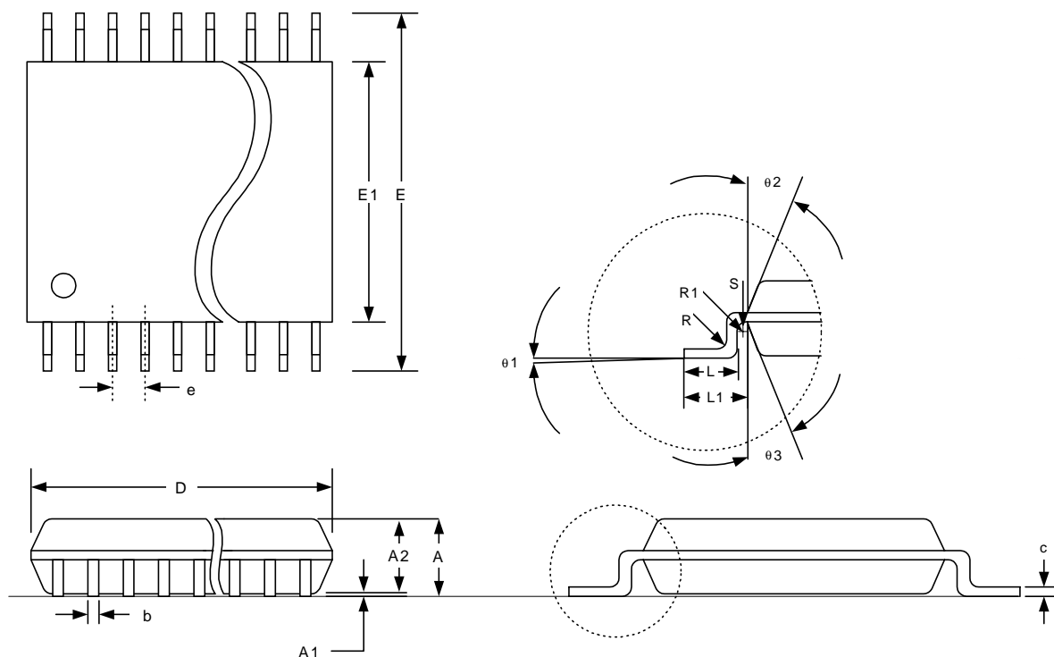
Figure 32. 16-pin Thin Small Shrink Outline Package (TSSOP)
